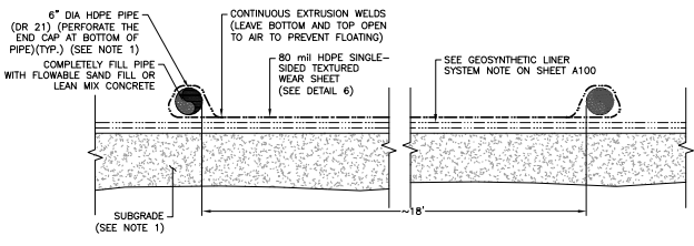
L POND WEAR SHEET BALLASTING A140 A150
