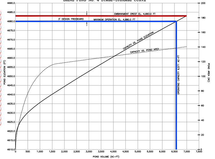
BRINE POND NO. 4 STAGE-STORAGE CURVE
