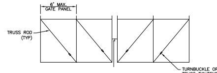
FRAME CONSTRUCTION GATES OVER 12'-0" TO 24'-0" OPENING
