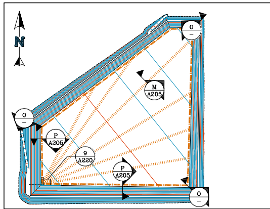
LCRS PIPING AND SUMPS
