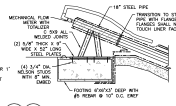
V PCMS AND LCRS SUPPORT AND ANCHOR DETAIL
