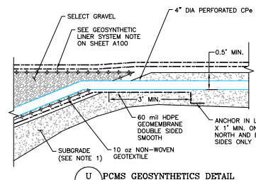
U PCMS GEOSYNTHETICS DETAIL
