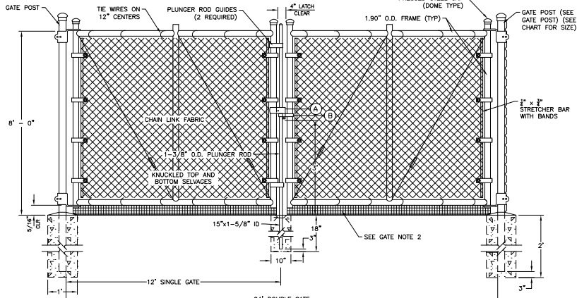
SWING GATE
